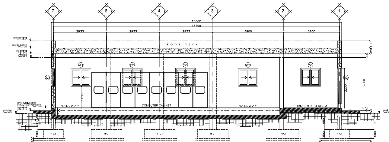
CONTROL ROOM SECTION THRU "AA"
