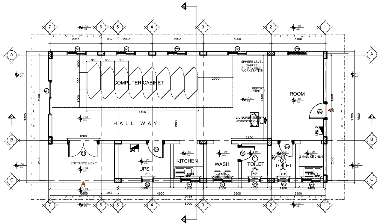
CONTROL ROOM GROUND FLOOR PLAN
