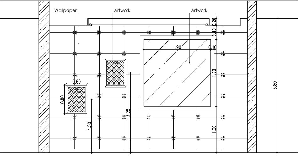
ELEVATION 3 VIP MEETING ROOM GR-66
