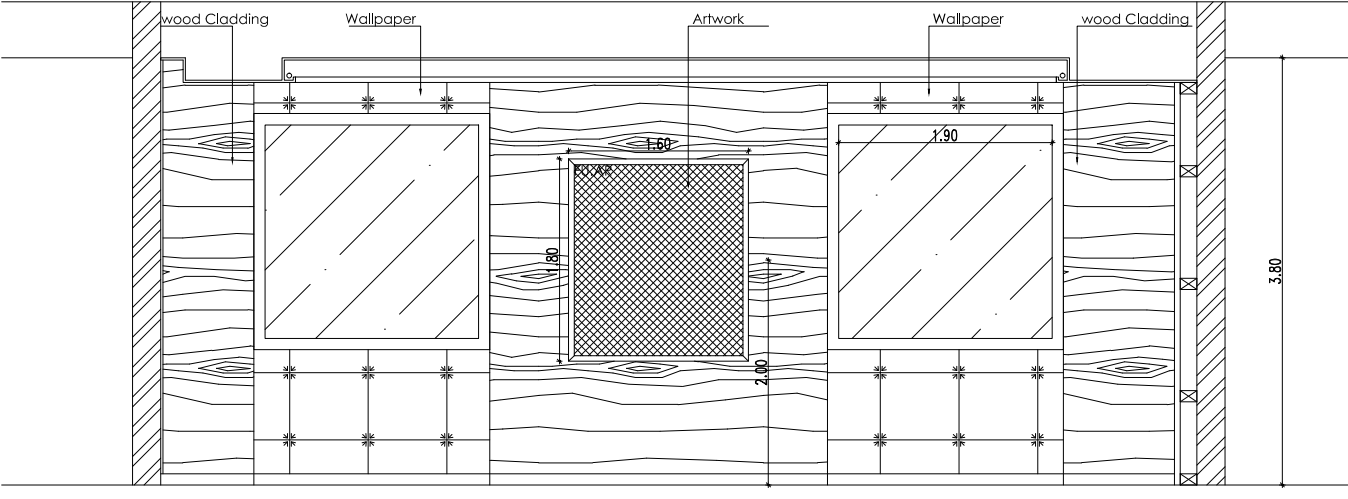
ELEVATION 4 VIP MEETING ROOM GR-66
