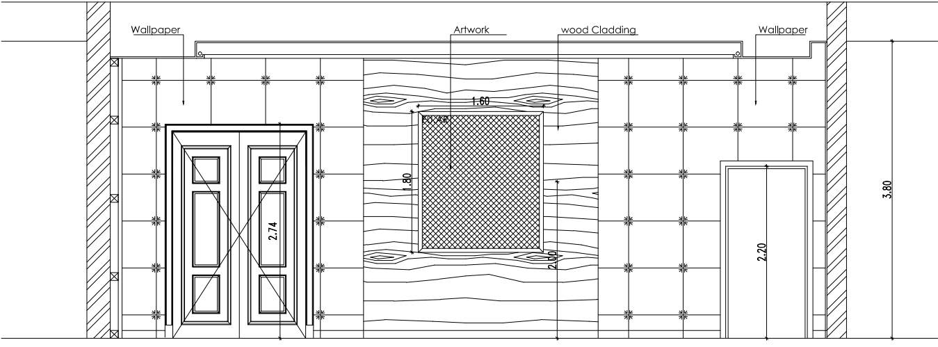
ELEVATION 2 VIP MEETING ROOM GR-66
