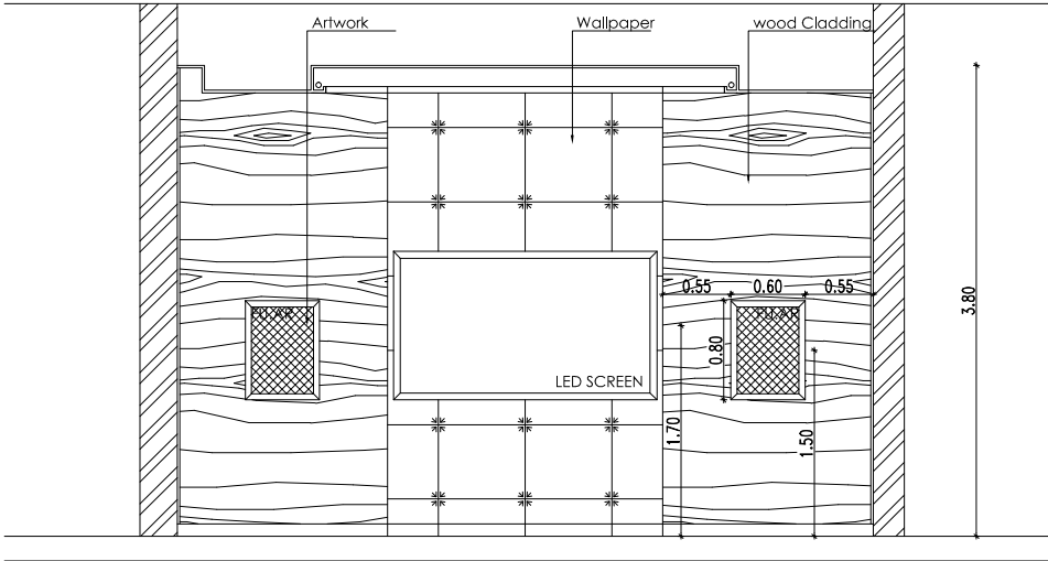
ELEVATION 1 VIP MEETING ROOM GR-66
